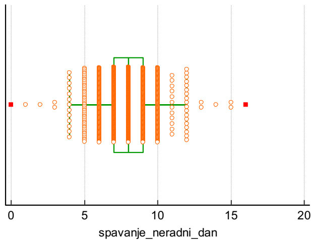
Box-and-Whisker plot
