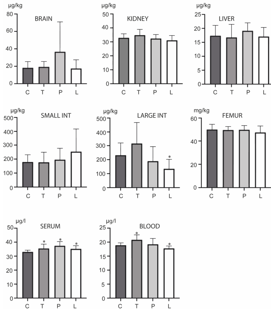
Figure 7. Concentrations of strontium in the brain, kidney, liver, small intestine, serum, blood and femur after the three-month oral administration of silicates. C denotes the control group; T denotes the experimental group receiving TMAZ; P denotes the experimental group receiving PMA; and L denotes the experimental group receiving Ludox silica. Asterisk (*) denotes significant differences between the experimental groups, with control at p < 0.05 .
